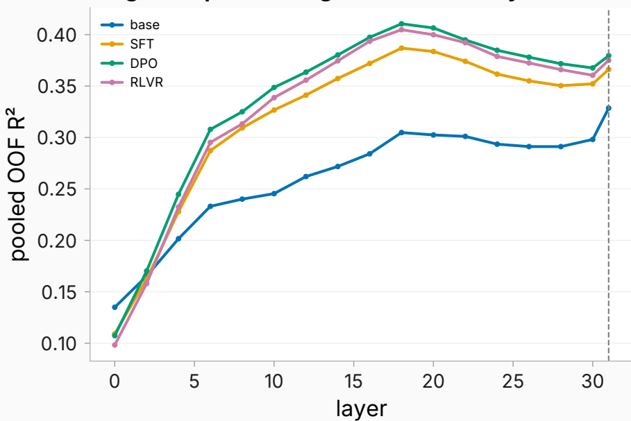
single corpus — diagonal ctx-arm layer curves
