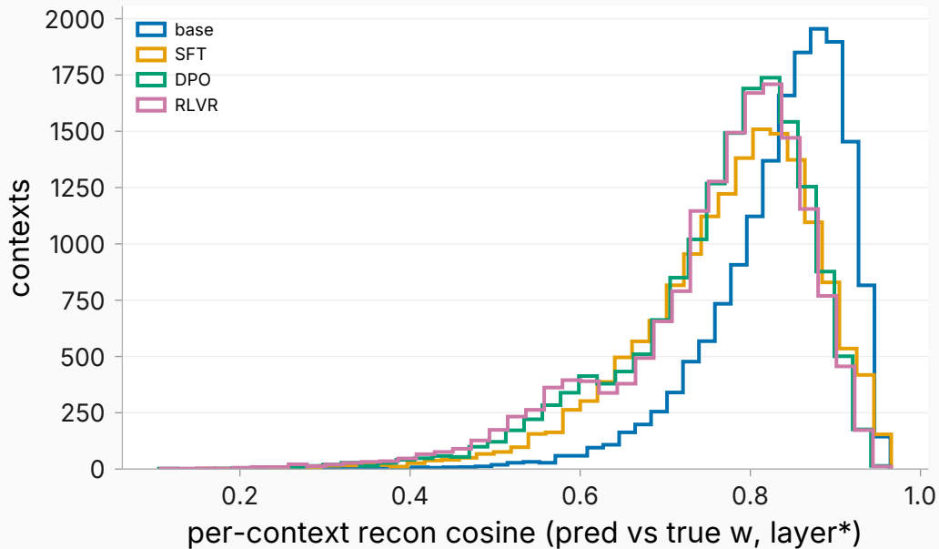
Per-context reconstruction cosine (single corpus)
