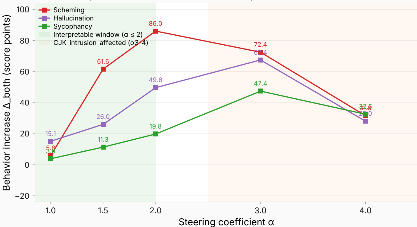
Dose ladder: behavior strength vs. steering coefficient (raw draws; delta from neither-arm baseline, all traits)
