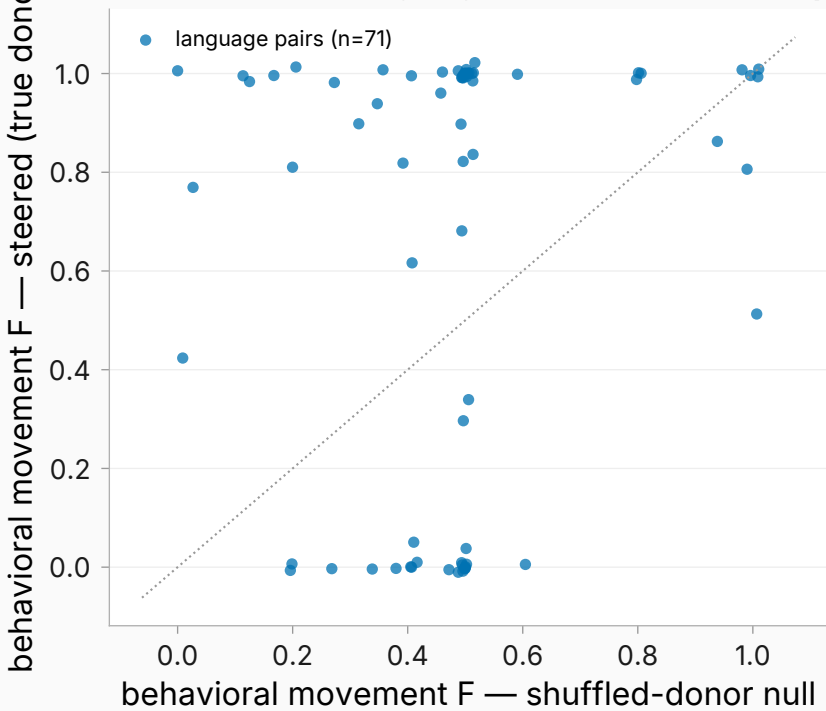
Qwen3.5-9B, language cells: three-token prefill, patch-content donors — per pair
