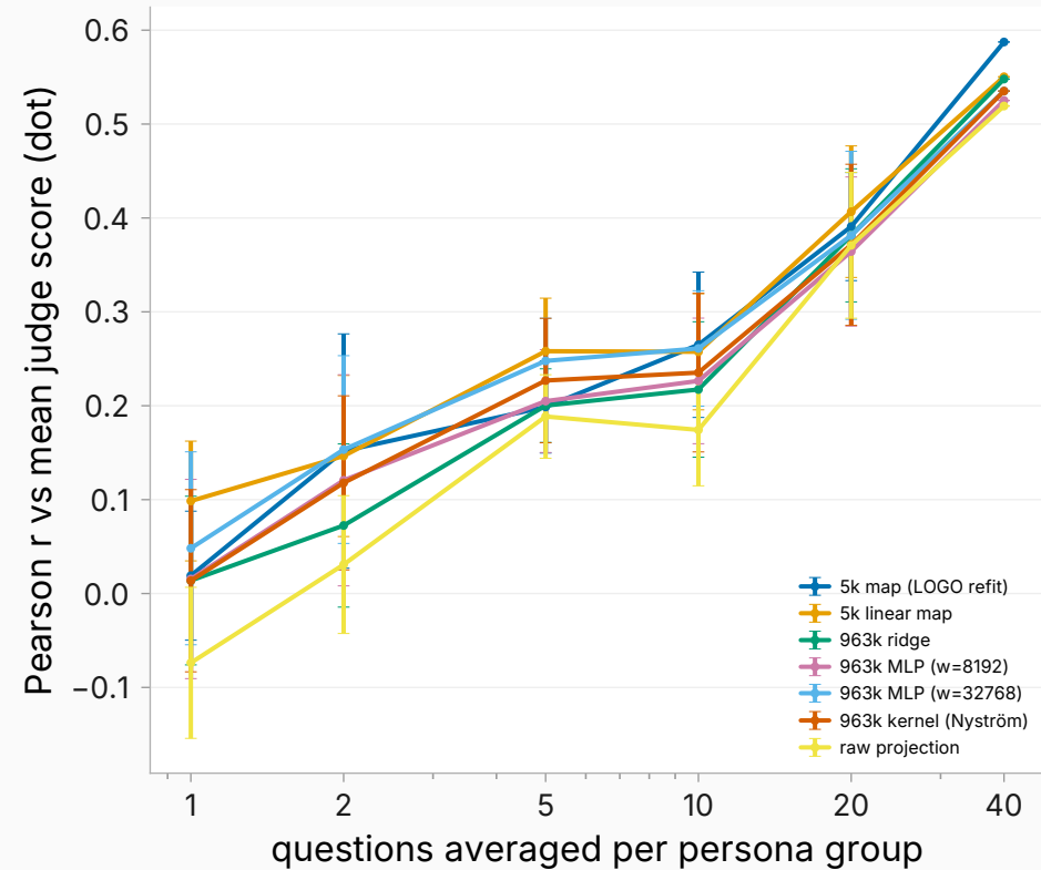
hallucination (L19)
