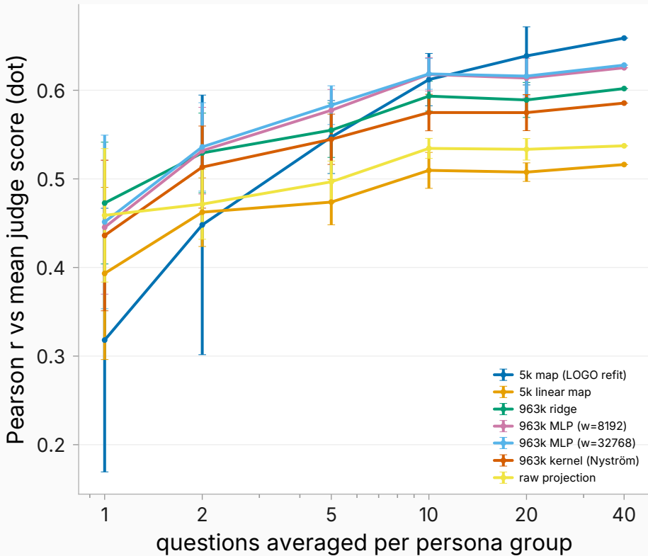
evil (L14)
