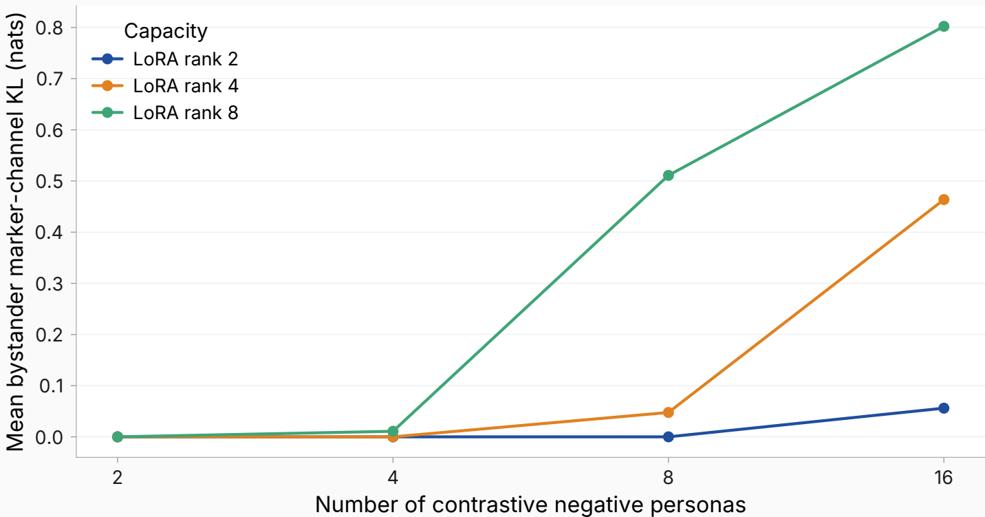
Bystander leakage rises with negative count, in lockstep with source implant
