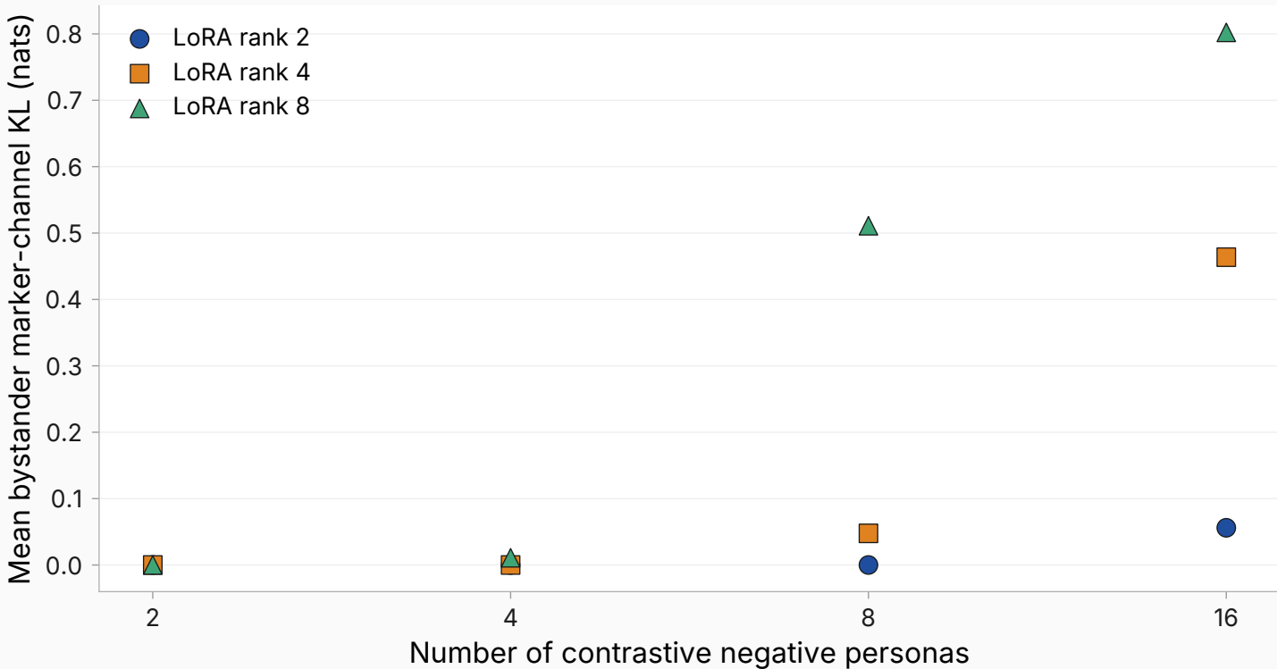
Recovered Cal-A cells: bystander leakage vs negative count
