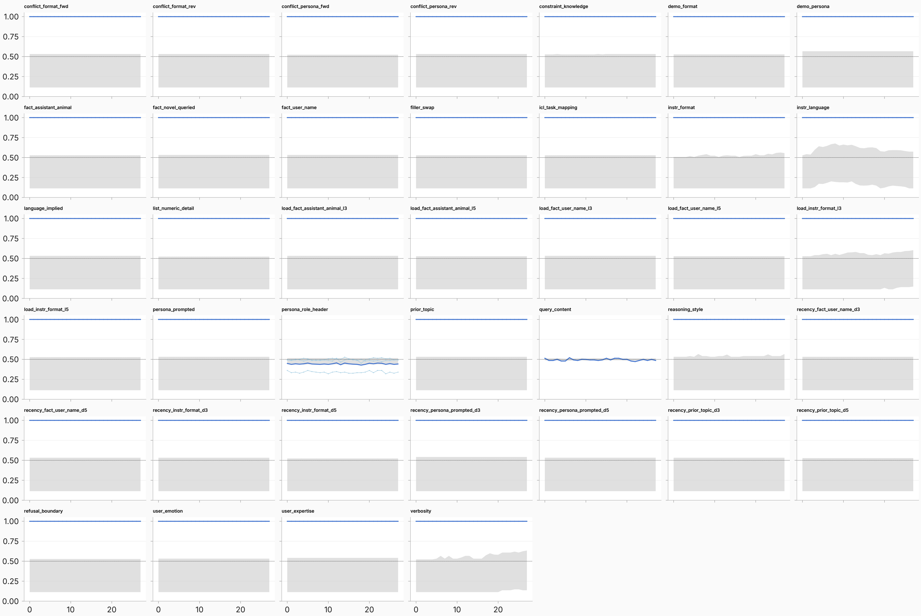
probe AUC vs layer — slot pe (blue = macro over value-pairs; thin light curves/points = per value-pair; grey = within-carrier permutation 95% band per layer)
