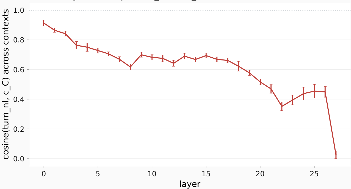
Boundary-triviality: turn_nl vs c_C (mean +/- std over contexts)
