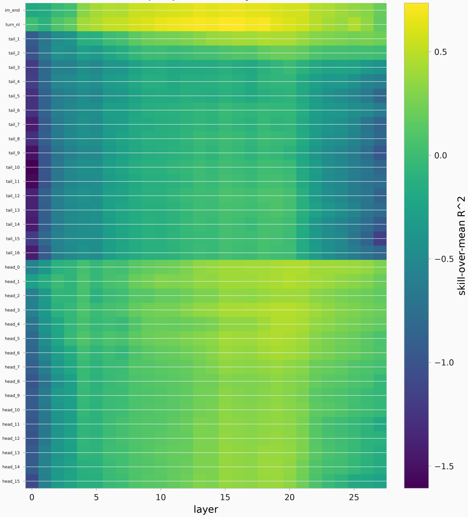
Reconstruction R^2 per position x layer
