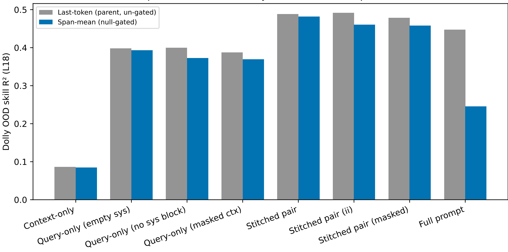
Corpus-transfer OOD (Dolly) — last-token vs span-mean
