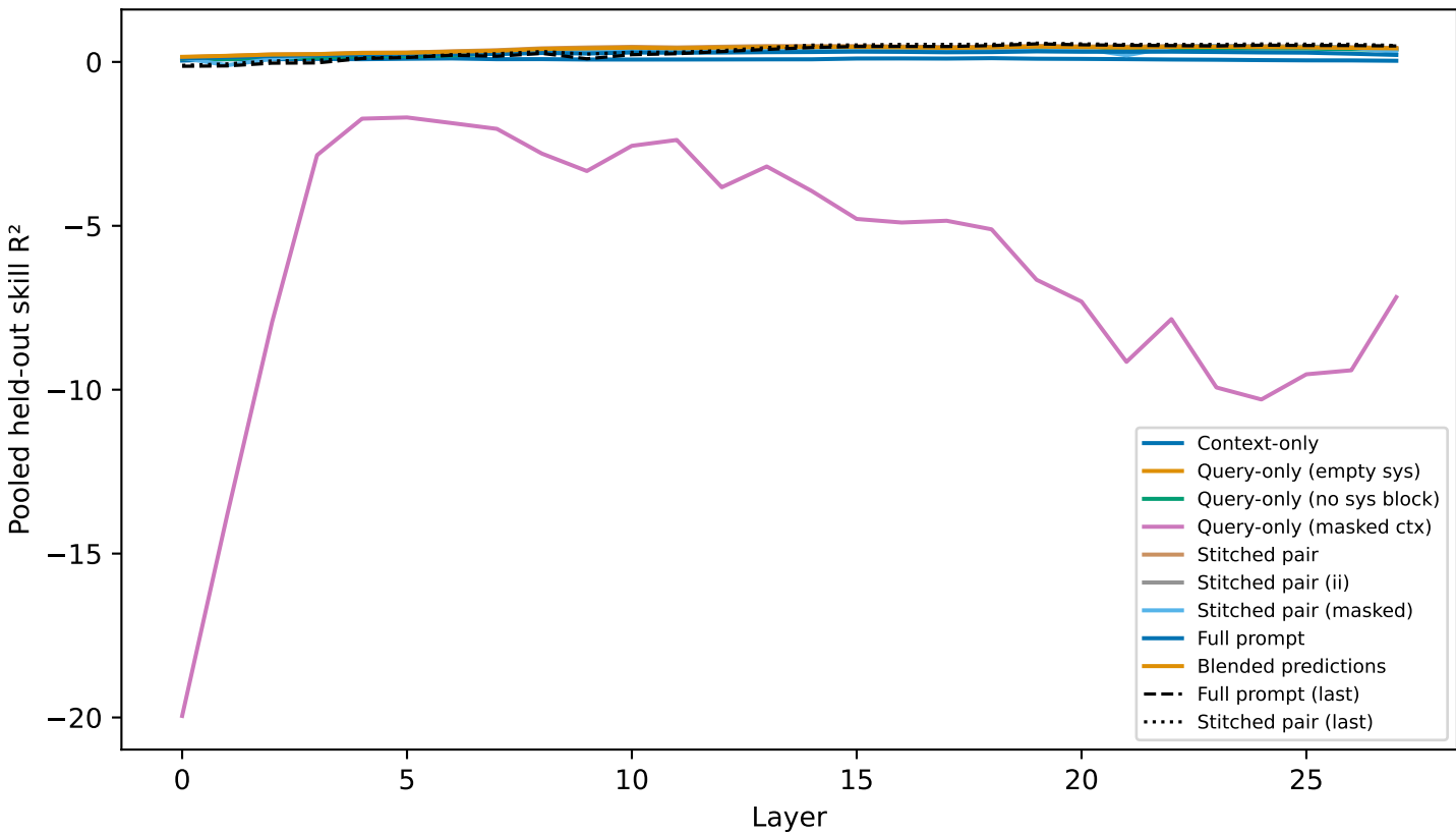
Layer sweep, span-mean features — betley
