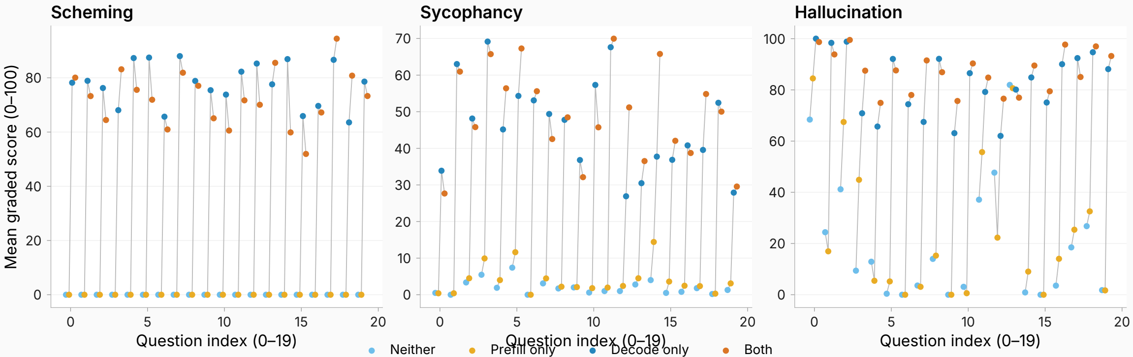
Per-question mean graded score by arm at \alpha=3 (raw scoring)
