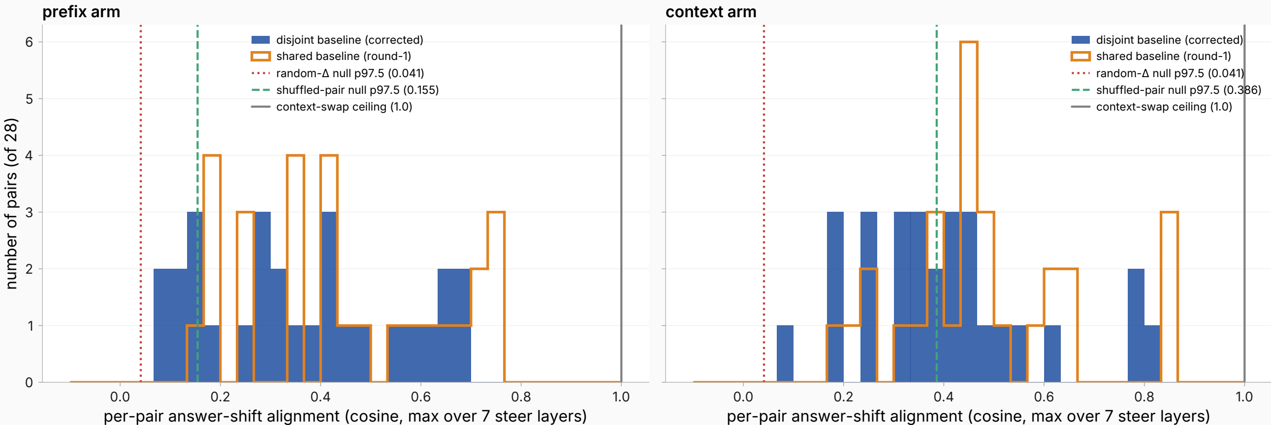
Observed per-pair alignment vs its nulls, before and after removing the shared-baseline noise term
