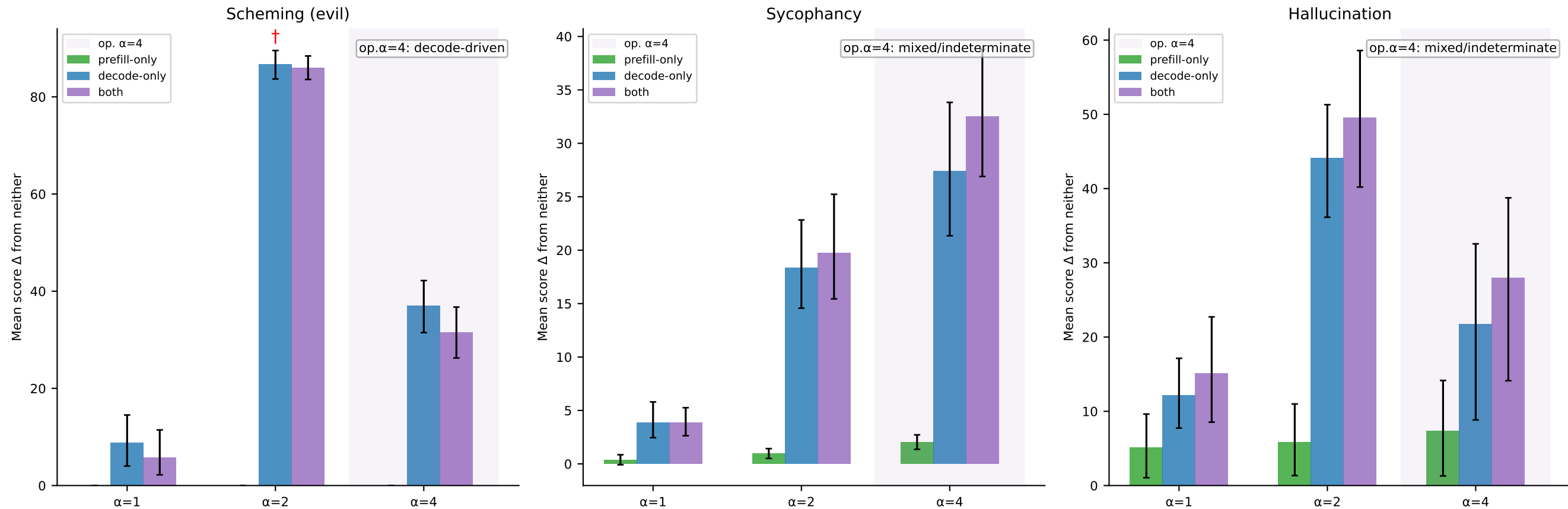
Alpha ladder: deltas by arm and \alpha level ( \dagger = K2 ceiling gate fired; shaded = operating \alpha )
