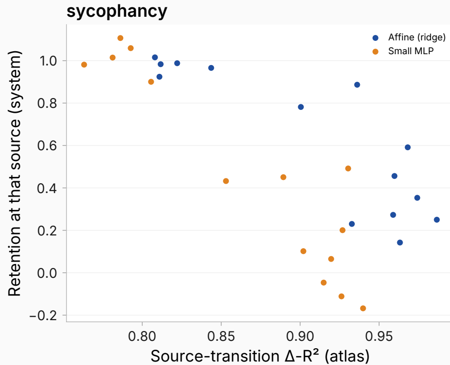
\Delta -R 2 vs behavior-retention divergence
