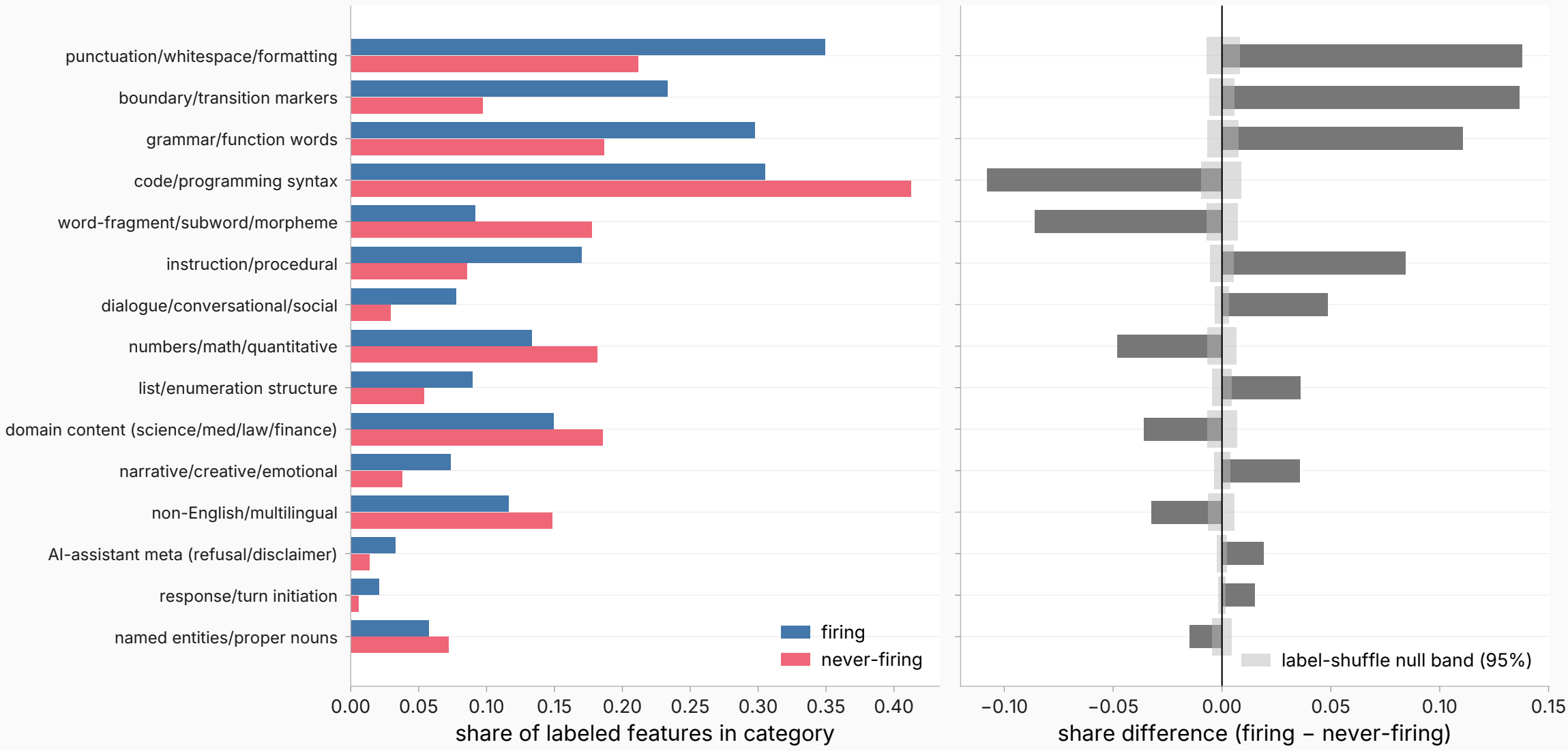
Answer-side description categories: firing vs never-firing features
