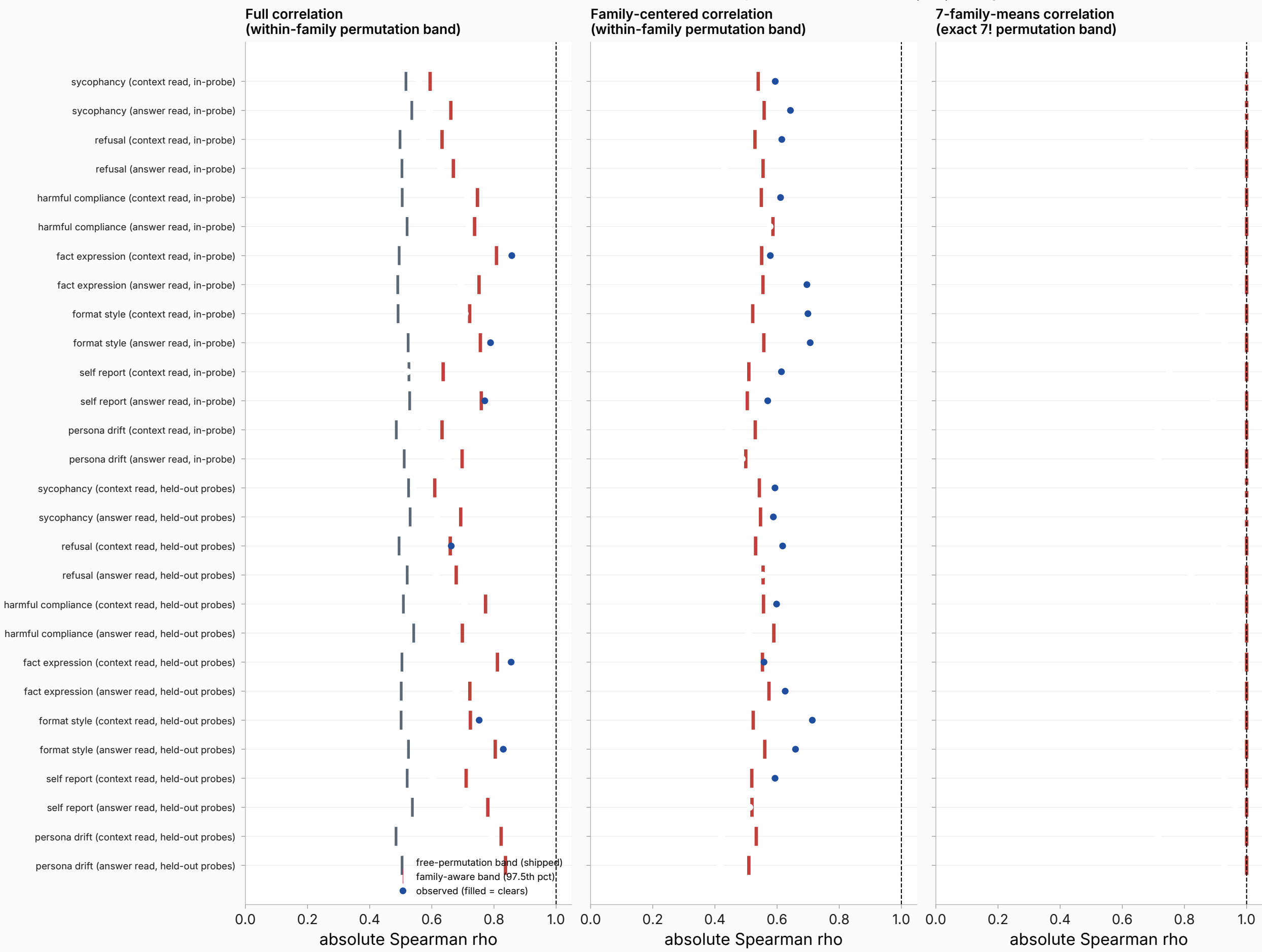
Behavior read-out vs family-aware null bands (max-over-cells inherited per draw; dashed line = |\rho| ceiling 1.0)
