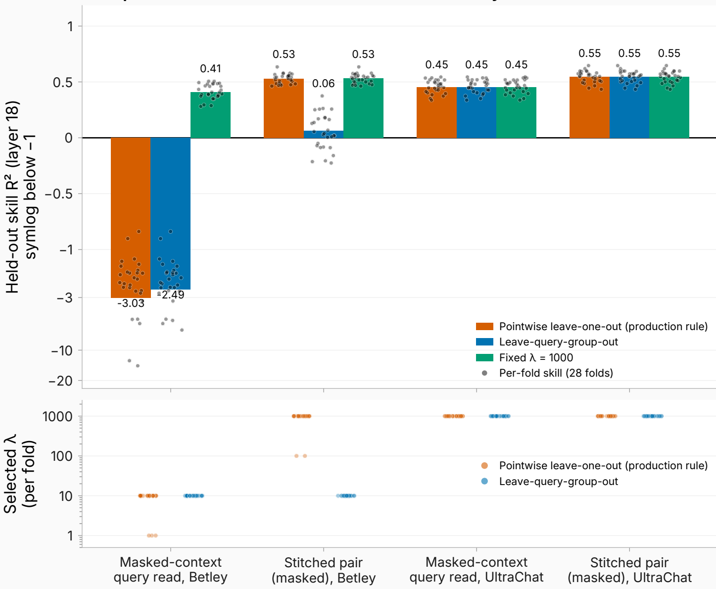
Group-level \lambda selection does not rescue the Betley masked-context read
