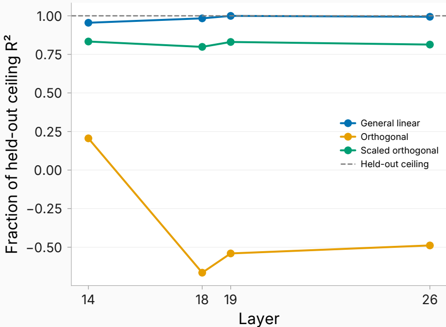
base rep \rightarrow instruct target
