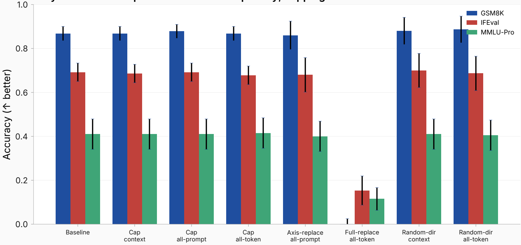
Only whole-state replacement wrecks capability; capping leaves it intact
