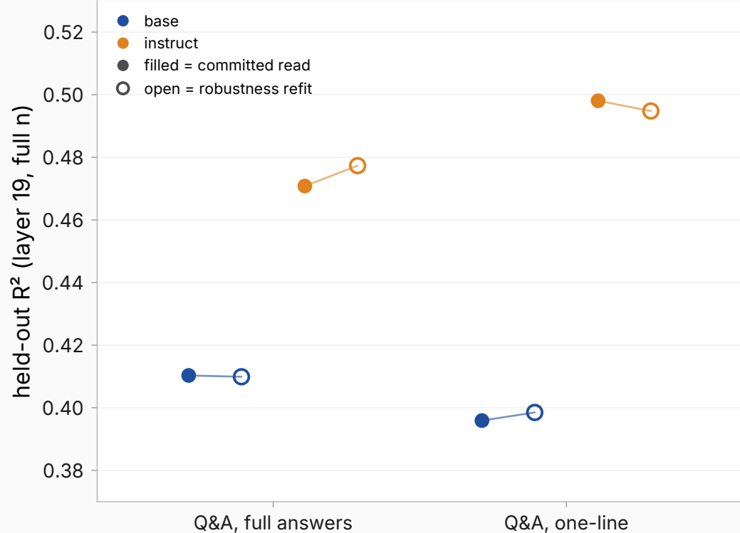
Multilingual-row exclusion on the Q&A rungs
