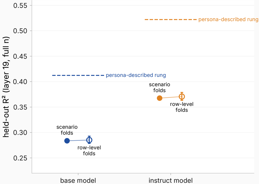
Fold granularity on the fiction-framed rung
