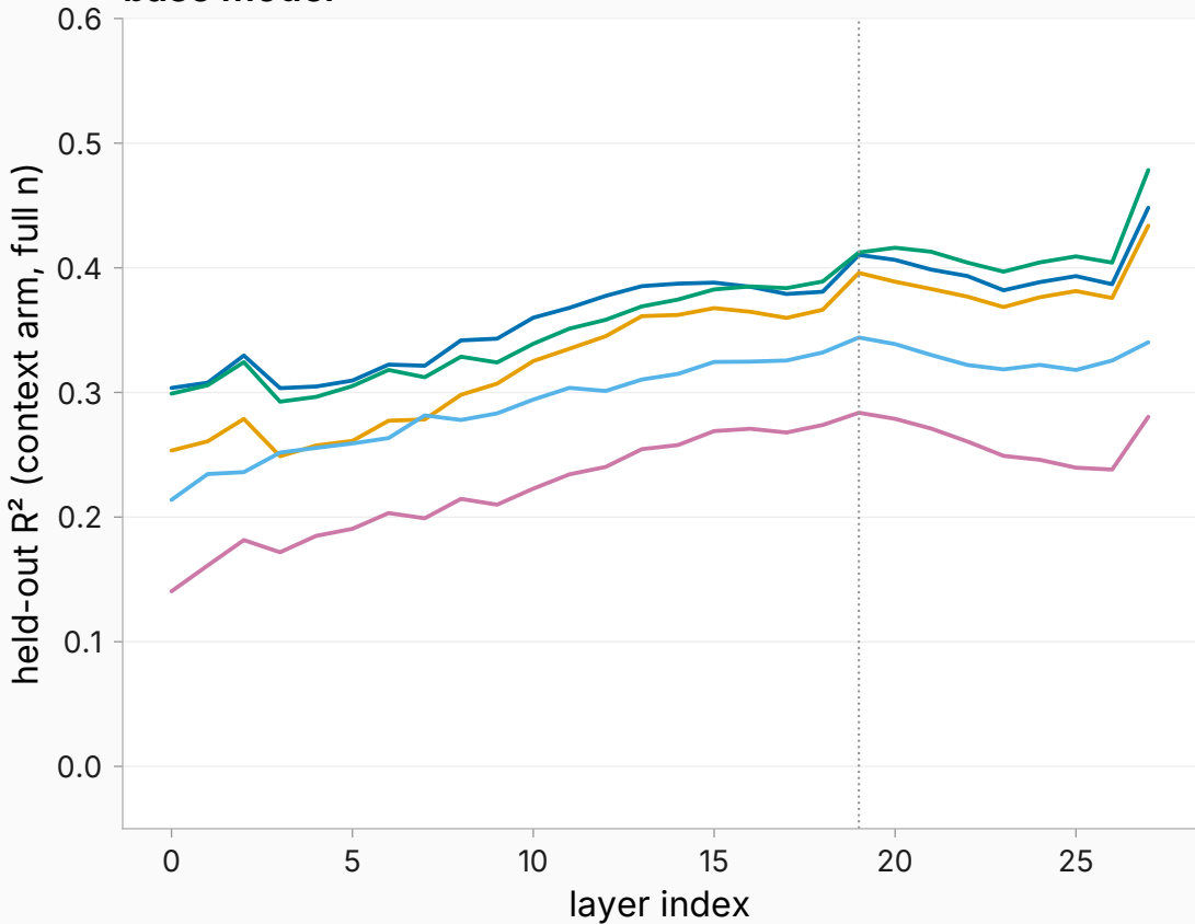
base model
