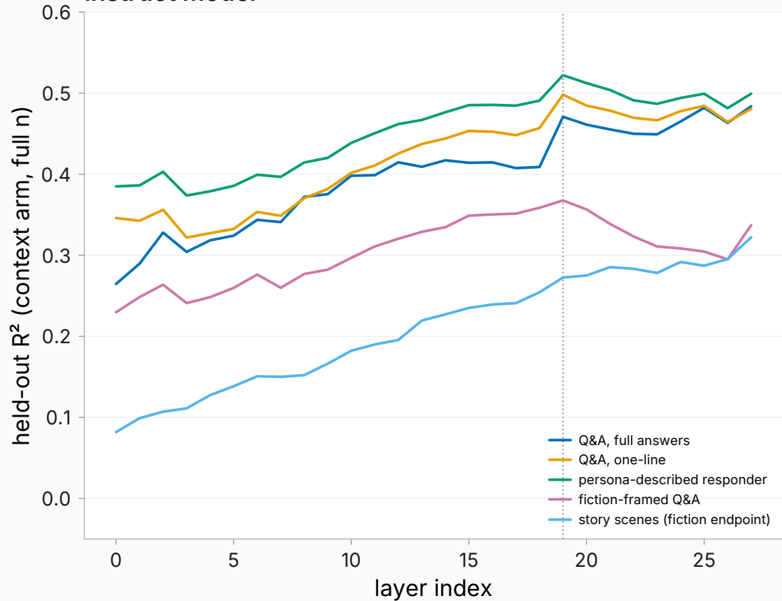
instruct model
