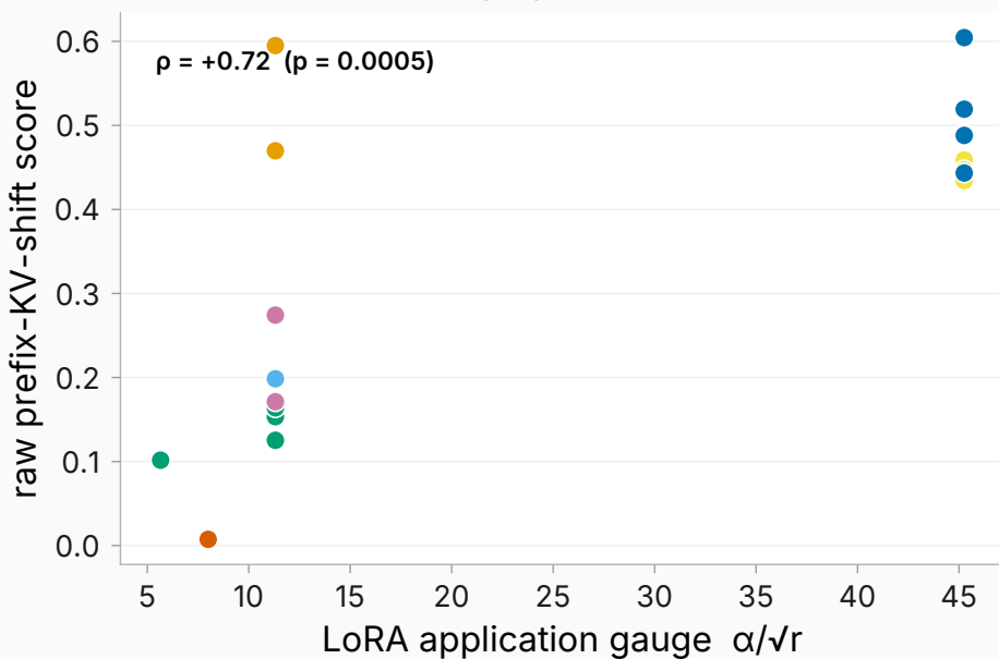
The raw score IS the LoRA gauge
