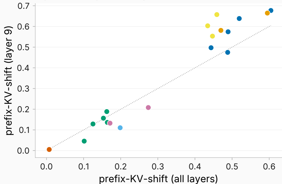
Layer-9 vs all-layer scores agree
