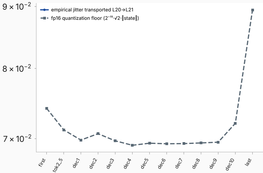
jitter-band anatomy — steered/context/L20
