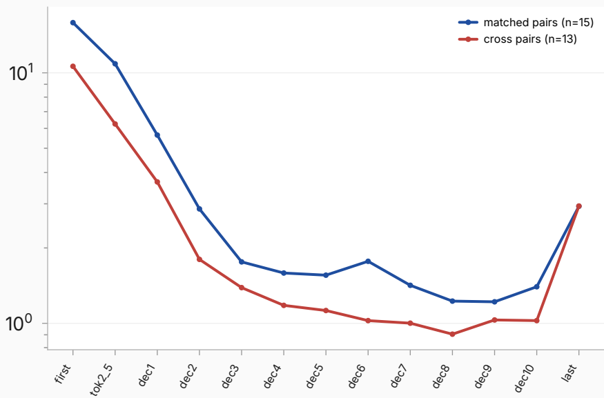
matched vs cross — steered/context/L14 (read L17)
