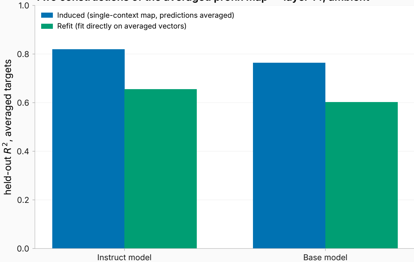
Two constructions of the averaged prefix map — layer 14, ambient
