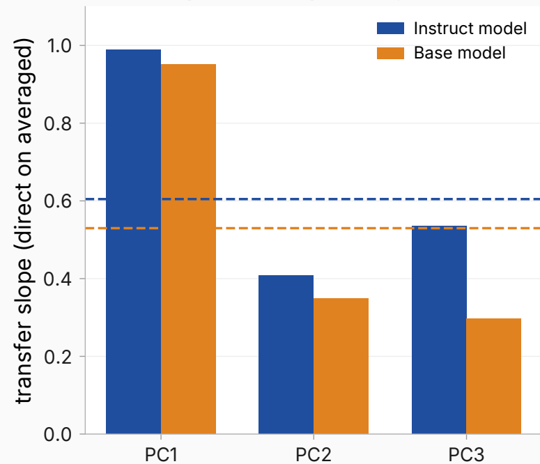
Per-component slopes vs global \alpha (dashed)
