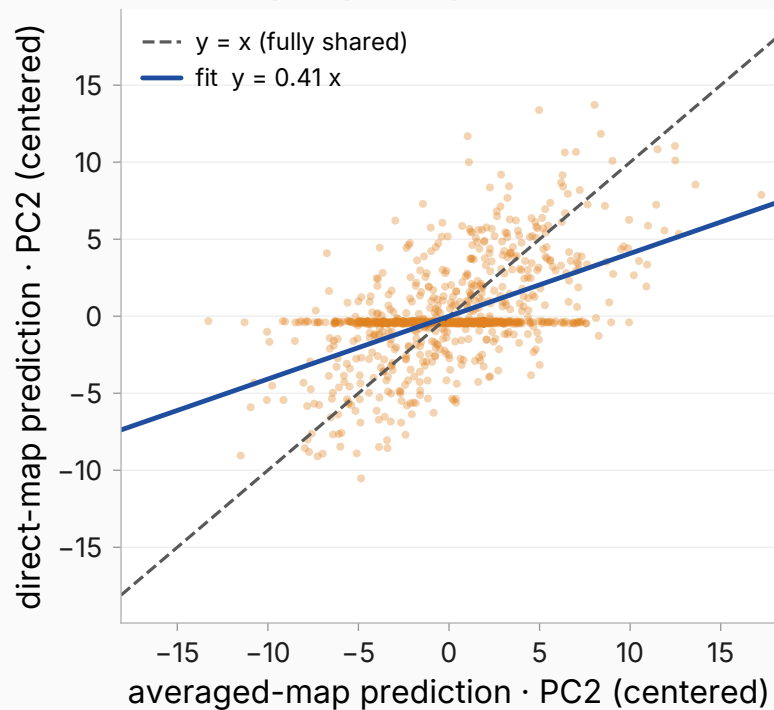
Instruct: per-prefix predictions on PC2
