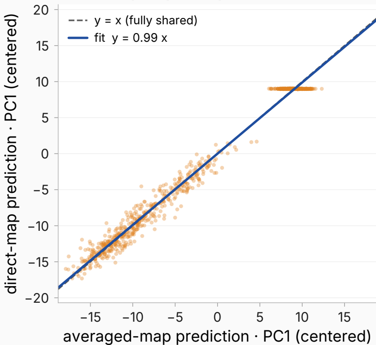
Instruct: per-prefix predictions on PC1
