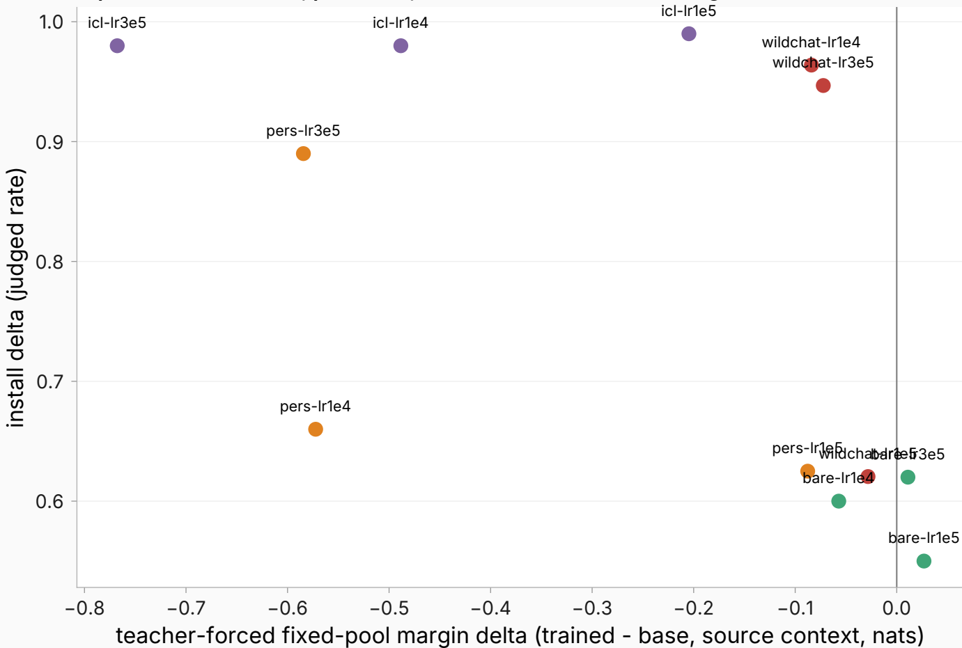
The fixed-pool margin ANTI-correlates with the judged install rate (Spearman rho = -0.72, p = 0.009, n = 12) - fails the rate-tracking validation
