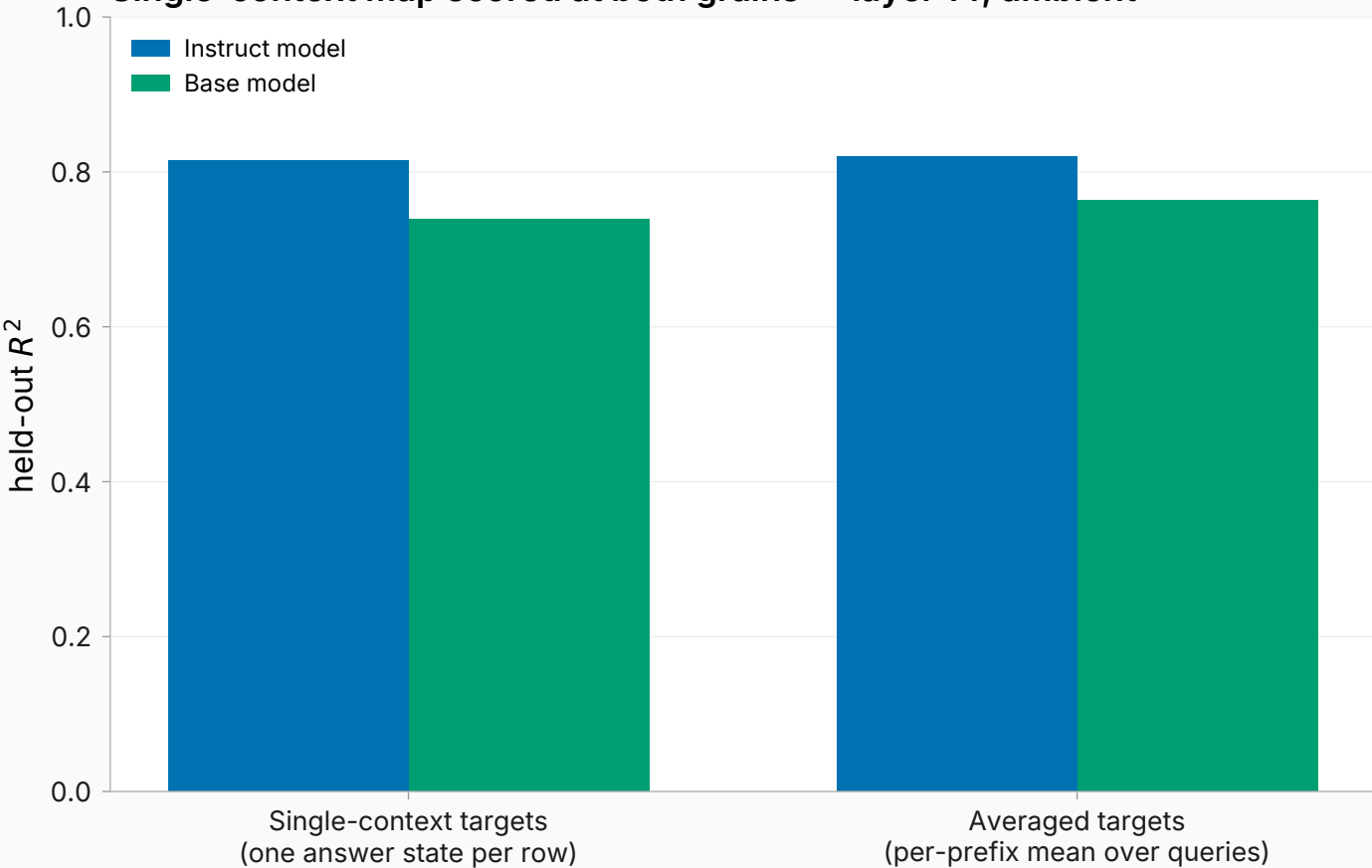
Single-context map scored at both grains — layer 14, ambient
