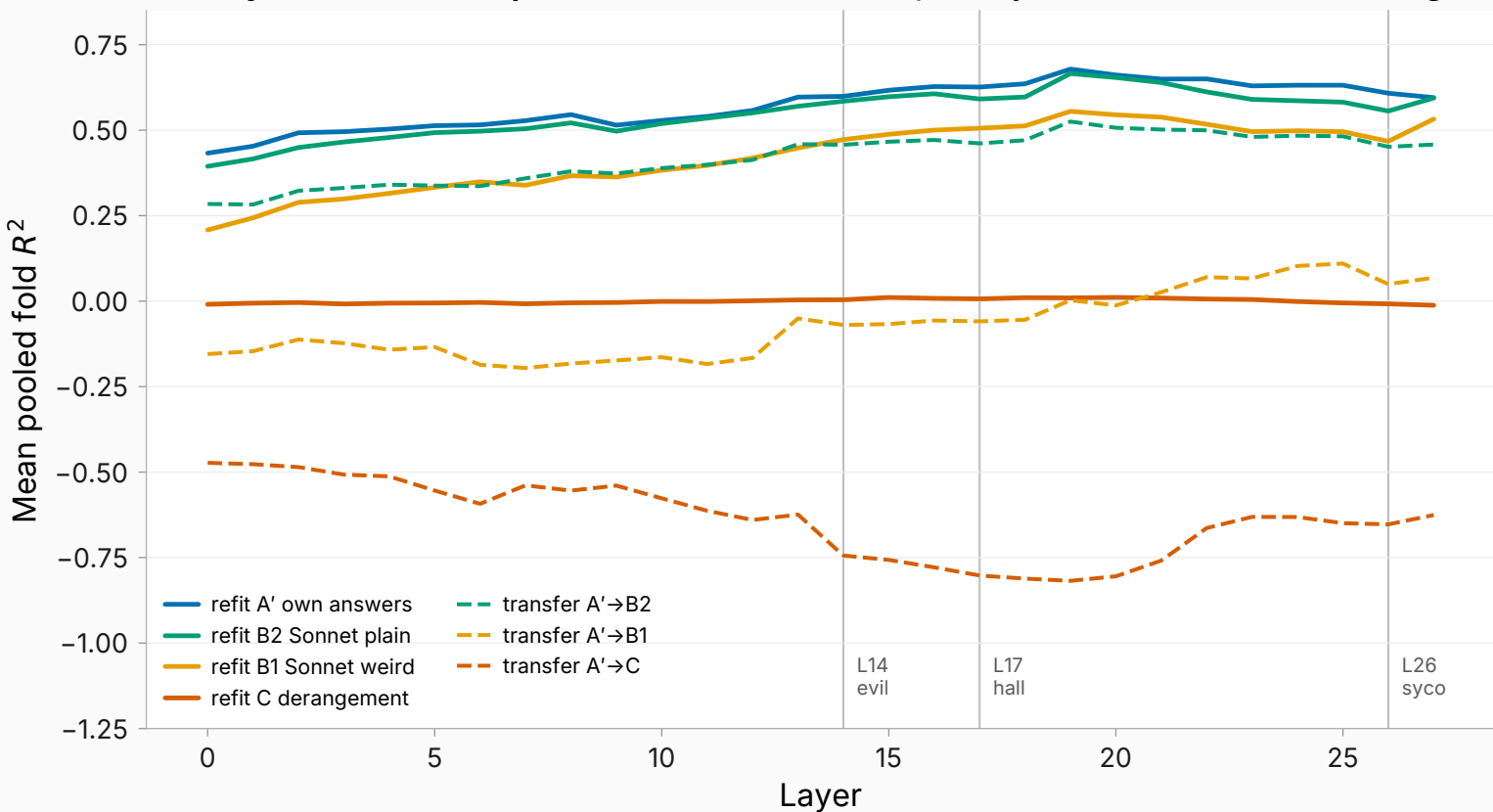
Per-layer R^2 : A'-fit map transfers to B2 (~75%), anti-predicts C (curves trait-agnostic)
