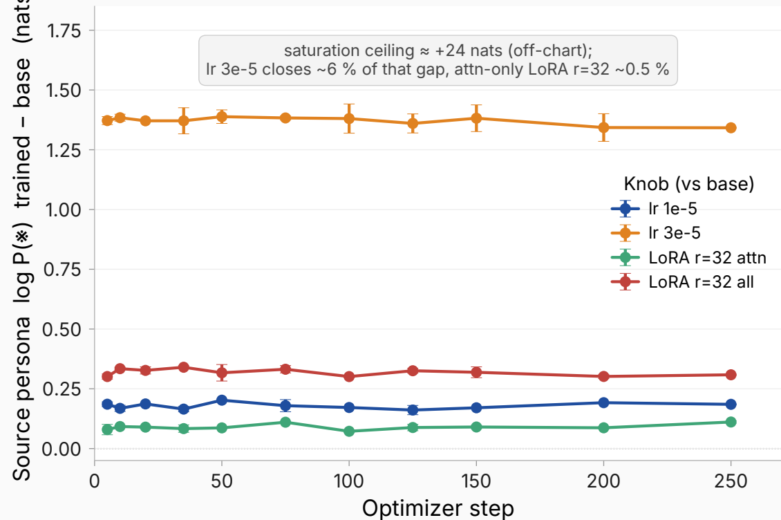
The loss IS moving log P(*) up — just not nearly enough
