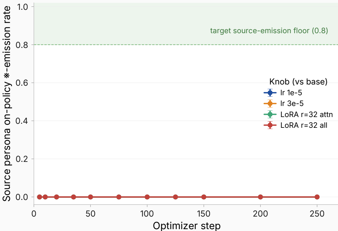
Source persona never emits *
