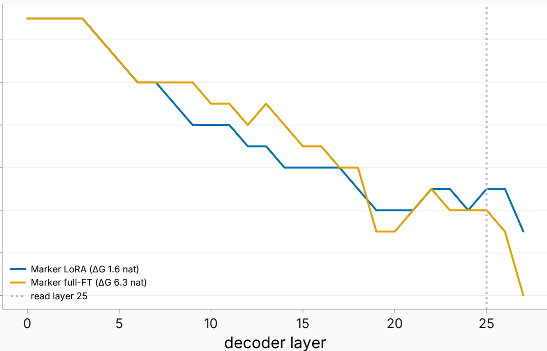
marker shift rank-k@90 — LoRA vs full fine-tune (response arm)
