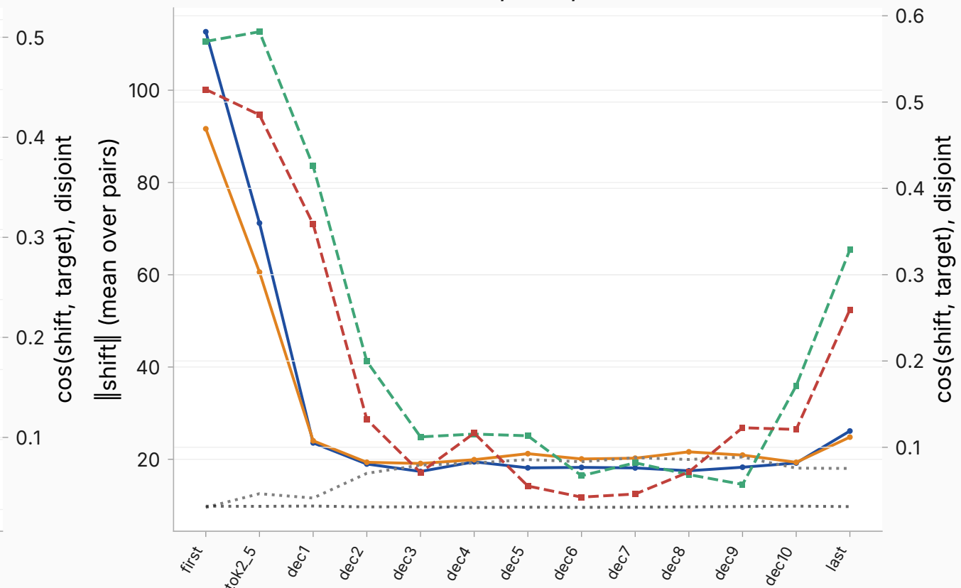
context · L20 ( \Delta=1.47 [1.38, 1.57]; width 0.10)
