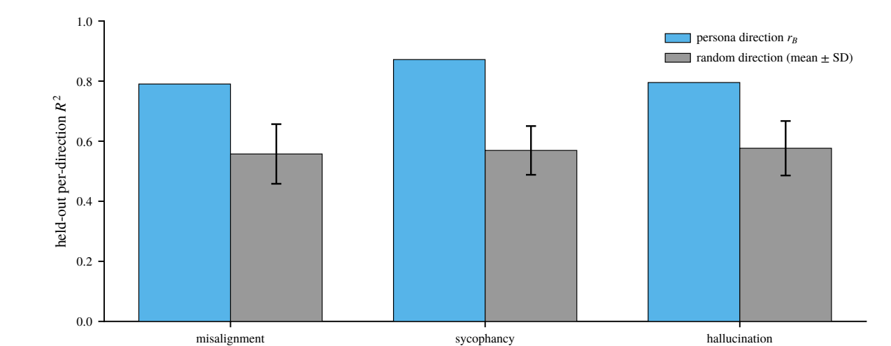
Figure 4. Held-out R^2 along the persona direction r_B against 50 random unit directions (mean \pm 1 SD). Fold 0 of 5; layers 14 / 26 / 17.
