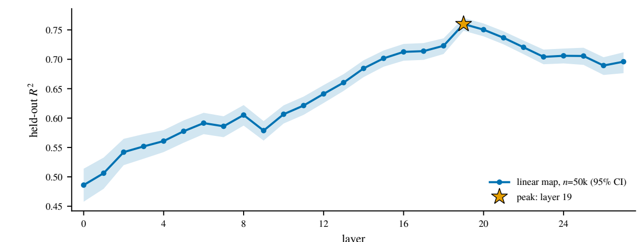
Figure 3. Held-out R^2 against the layer at which both v_C and v_A are taken (swept together). Band: bootstrap 95% CI over test rows. Star: argmax, layer 19 / 19 and 20 overlap. n_{\text{train}} = 50,000 , n_{\text{test}} = 1,000 .
