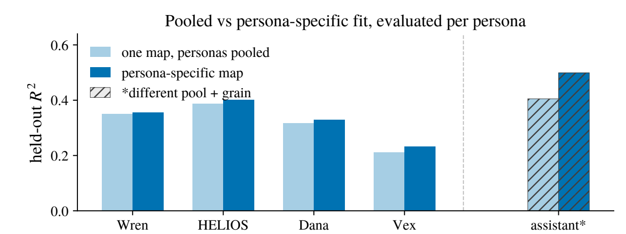
Figure 8. Held-out R^2 per character: one map pooled over all four (1,200 pts) against that character’s own 300-pt map. assistant* = separate lattice (rows, n = 4,375 ) reference only, not comparable.
