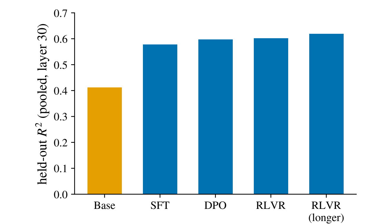
Figure 7. Pooled held-out R^2 at each stage of the Llama/Tulu ladder (layer 30), each stage fit and evaluated on its own on-policy answers.
