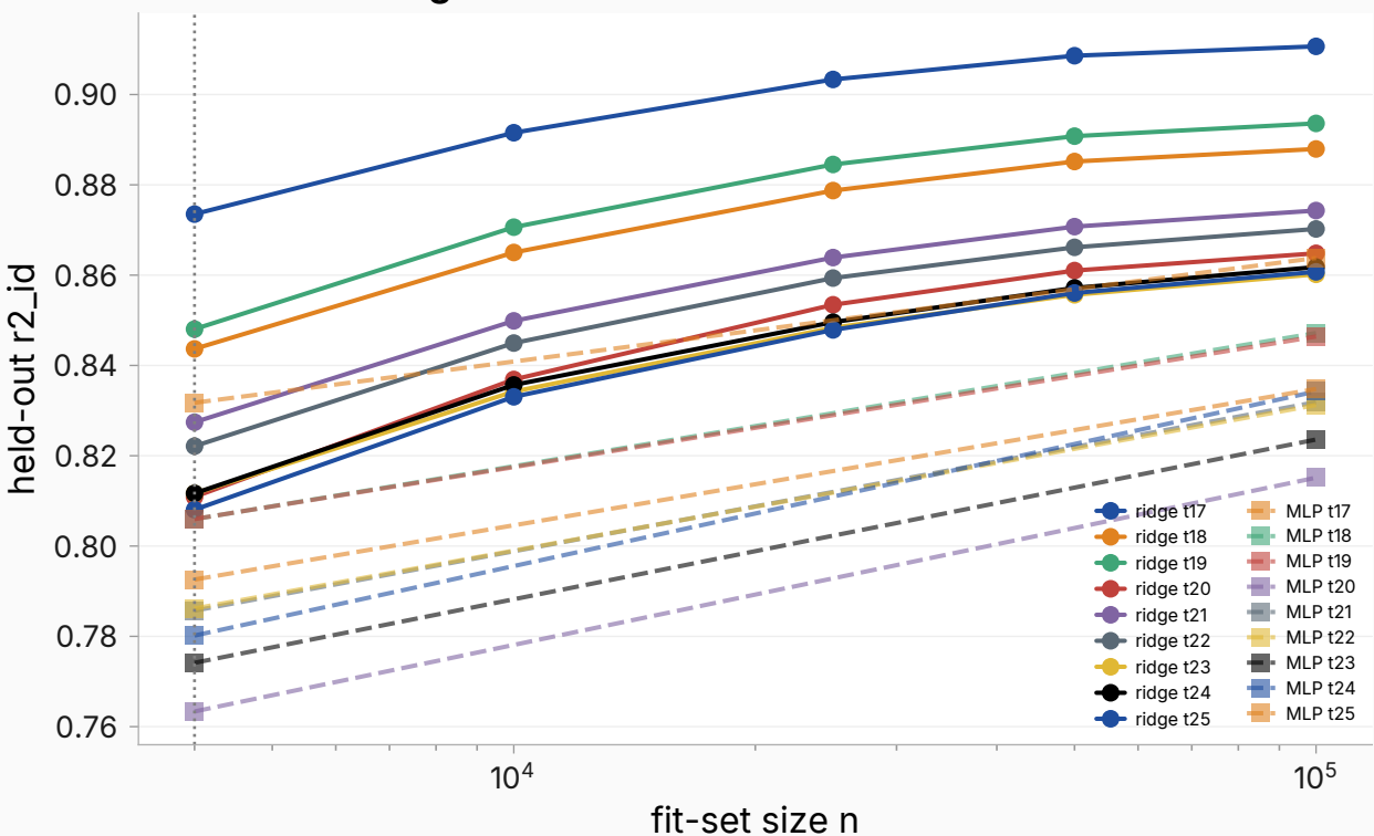
DV1 data-scaling curve — r2_id at data-limited transitions
