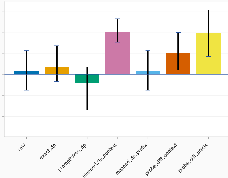
sycophancy (n=24 ds, 8 fam)
