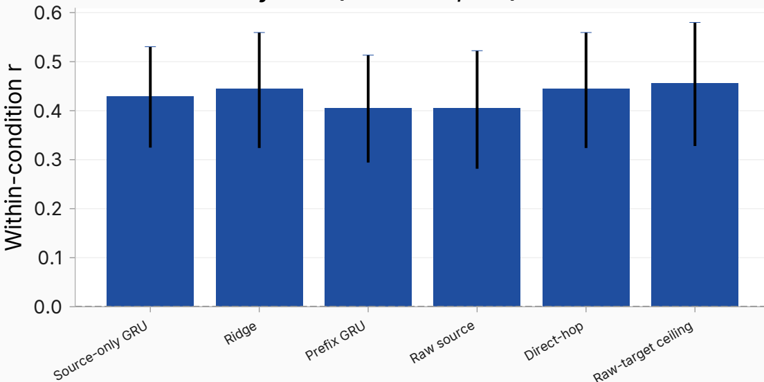
hallucination / system (source 16, k=1)
