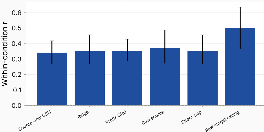
sycophancy / system (source 25, k=1)
