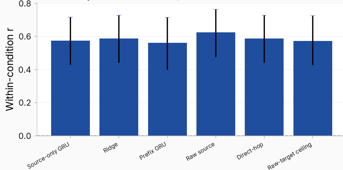
sycophancy / many_shot (source 25, k=1)
