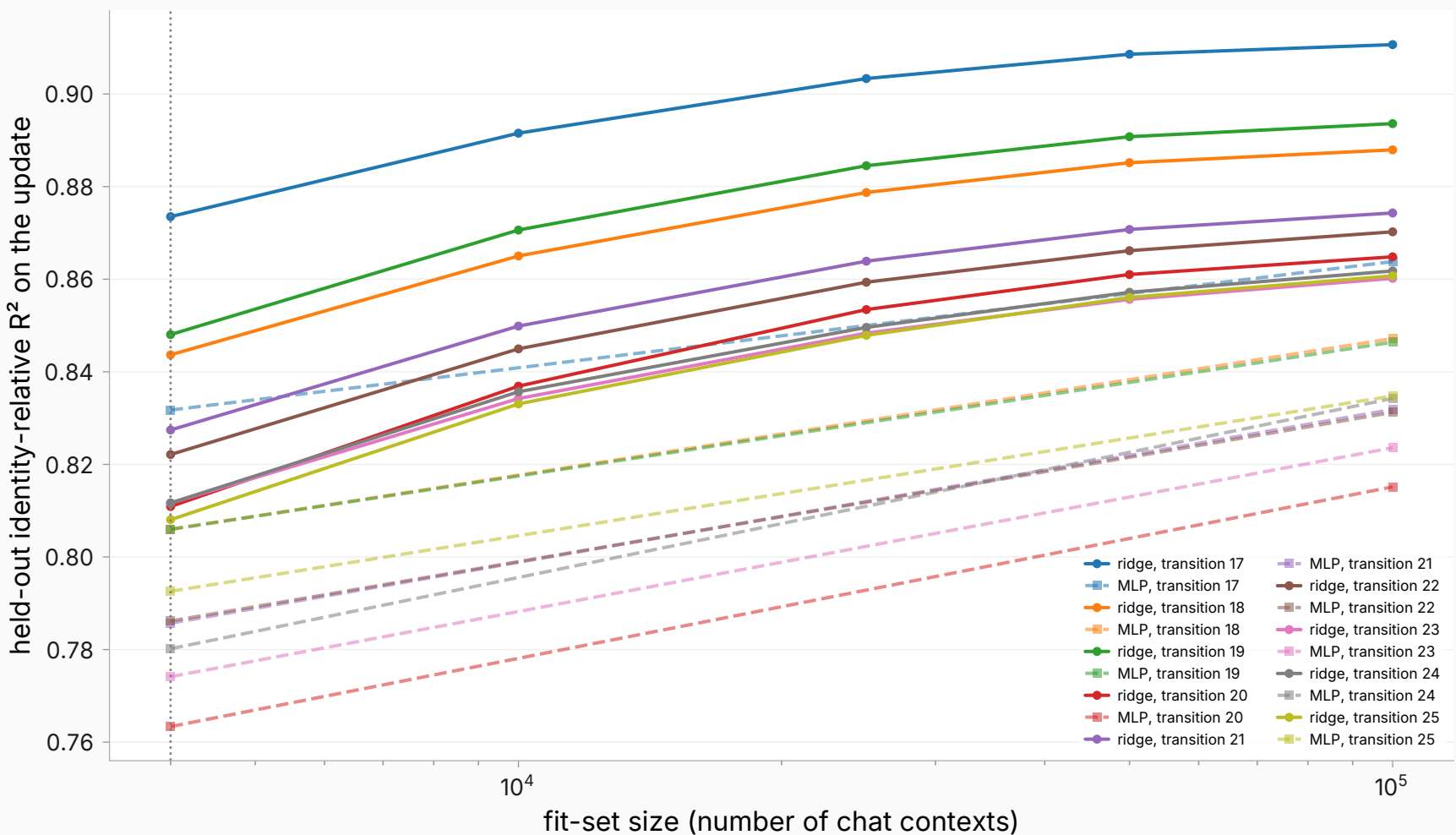
Late-layer update predictability keeps rising with fit data, decelerating
