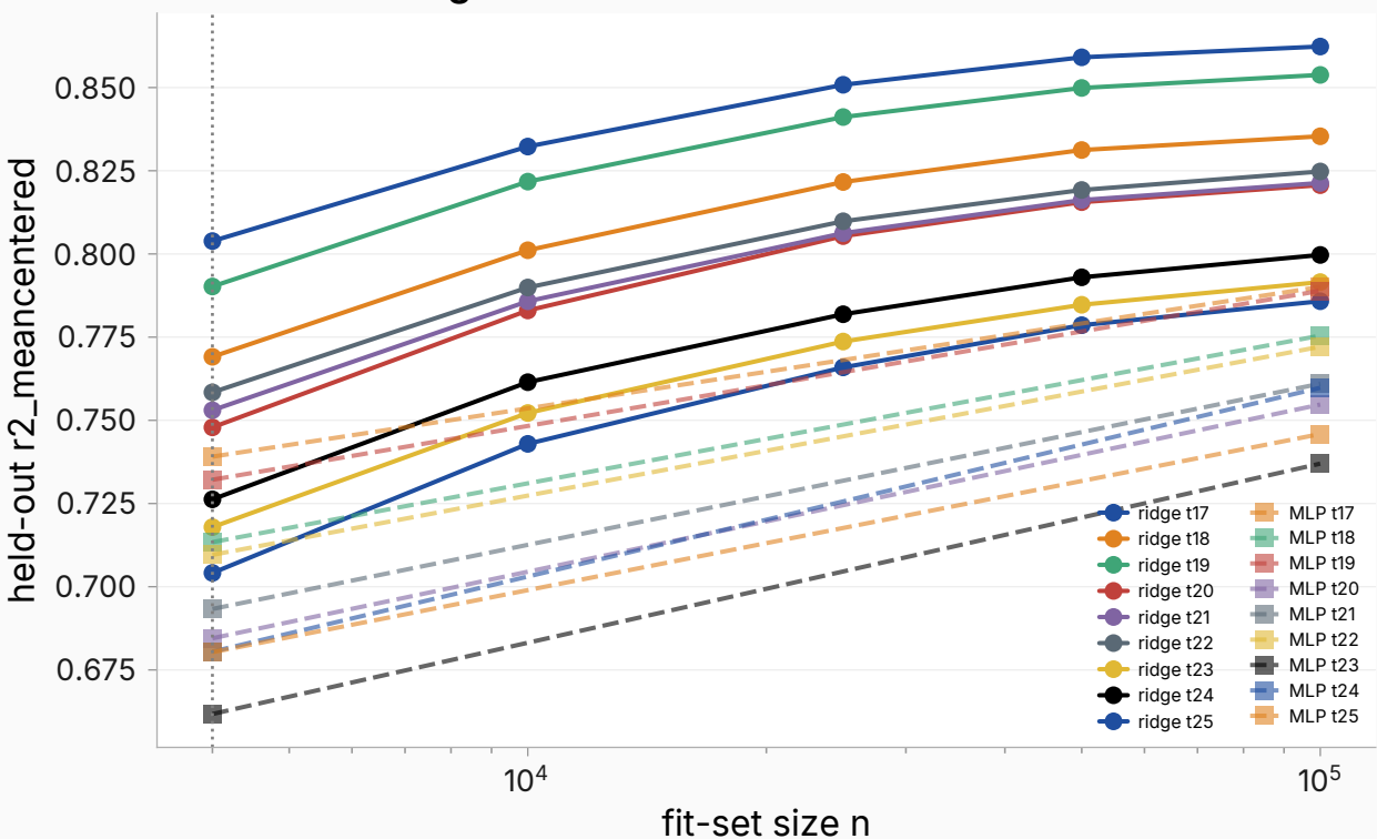
DV1 data-scaling curve — r2_meancentered at data-limited transitions
