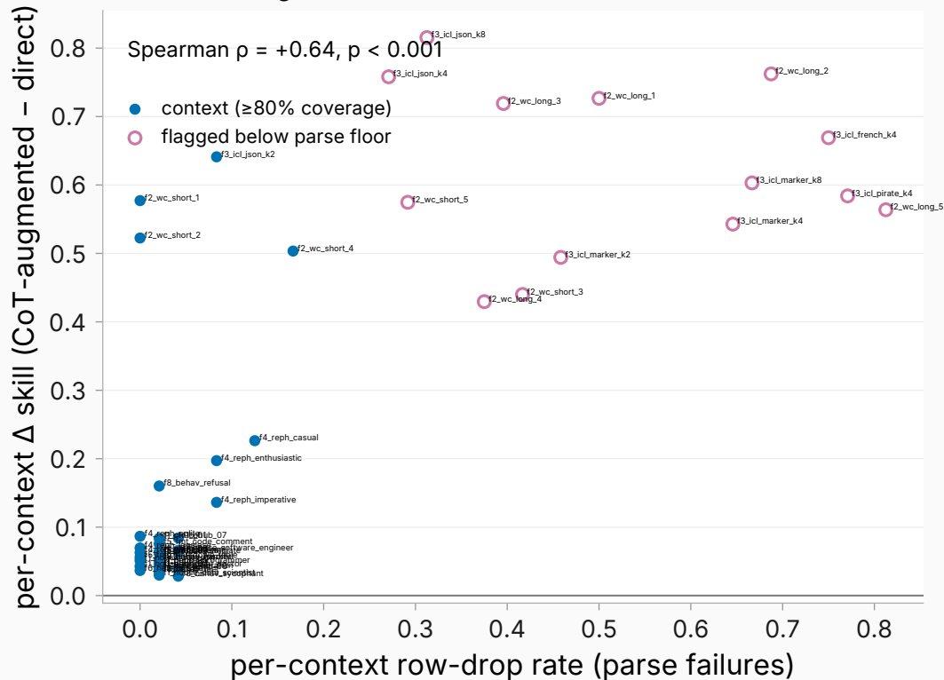
where the CoT gain concentrates
