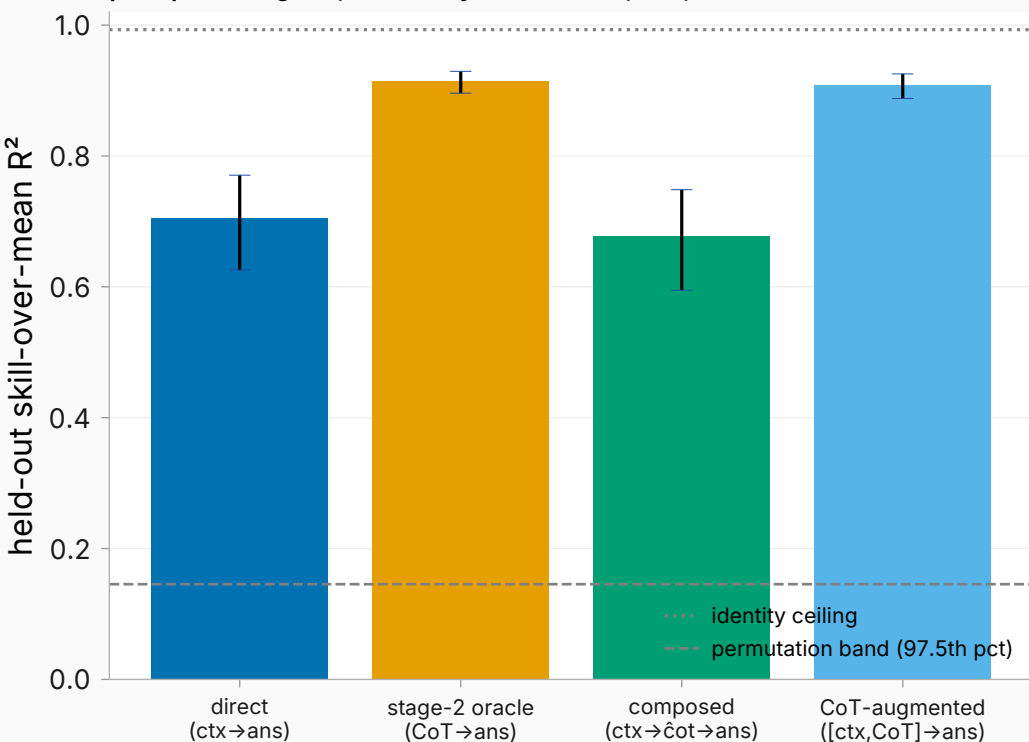
per-question grain, frozen layer 25 (LOCO, n=1,994 rows / 50 contexts)
