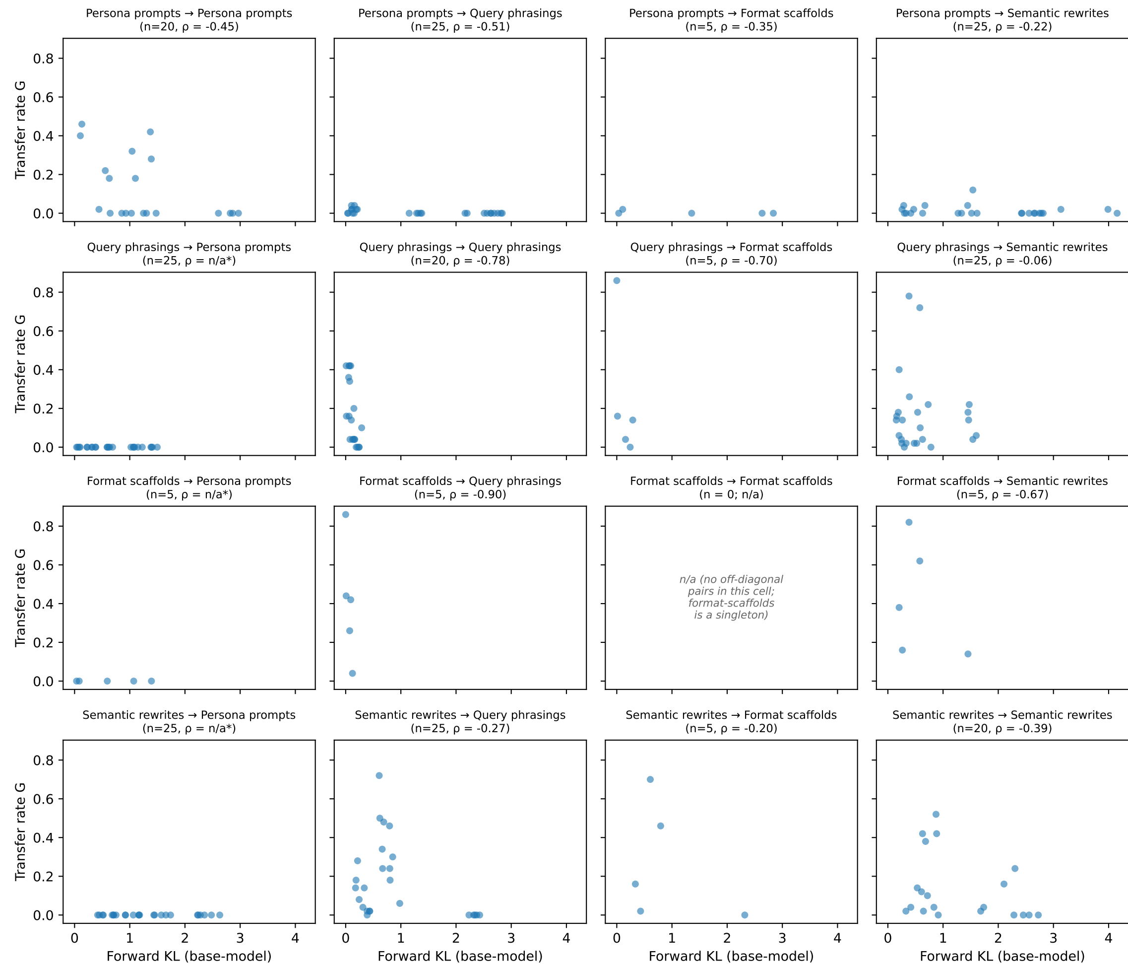
Per-(trained-class, eval-class) cell: base-model KL vs marker transfer rate (format-scaffolds class is a singleton — its self-cell has no off-diagonal pairs; \rho = n/a^* marks length-partial divide-by-zero in three small cells)
