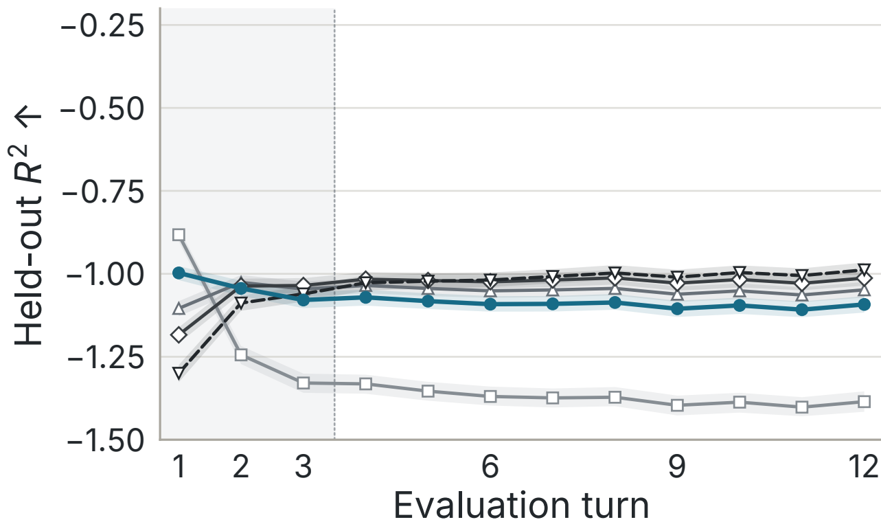
A · INSTRUCT
