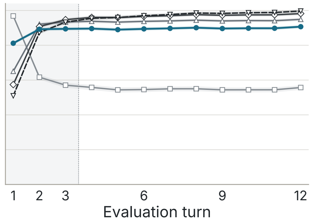
B · PRETRAINED
