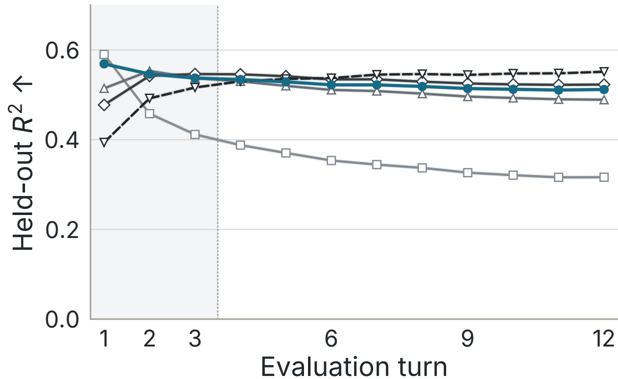
A · INSTRUCT
