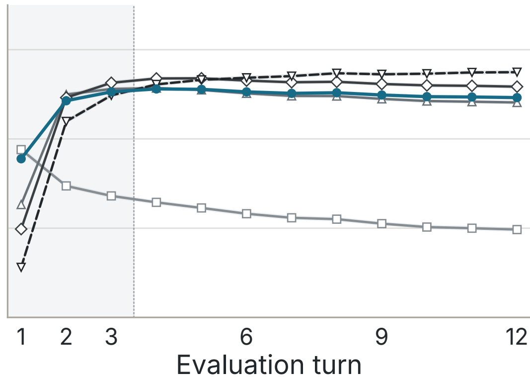
B · PRETRAINED
