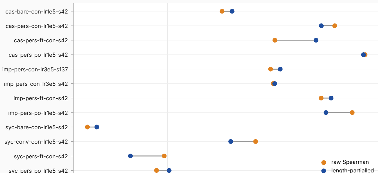
content arms: rho(p3b_tc, dv_change)
