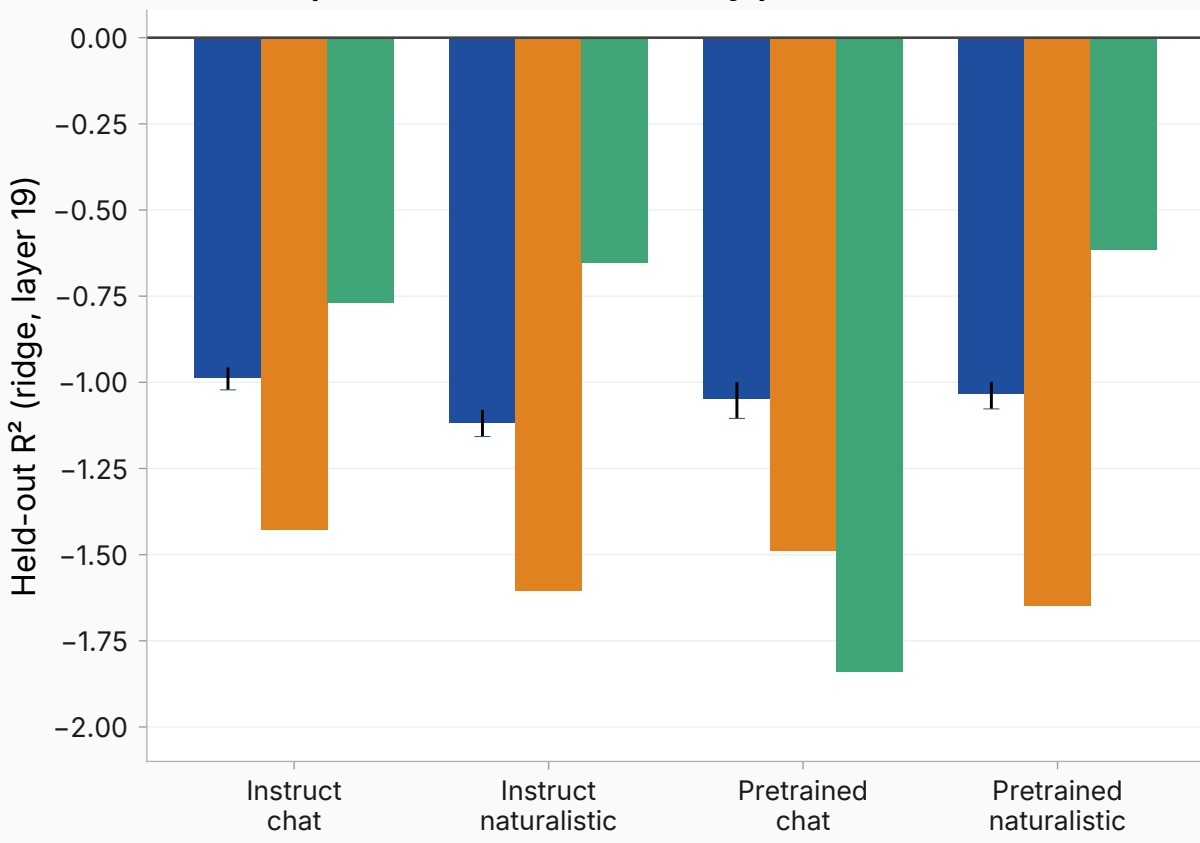
Linear map: below zero under every provenance
