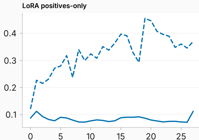
top-eigenvalue share of shift variance — own vs shared text (response arm)
