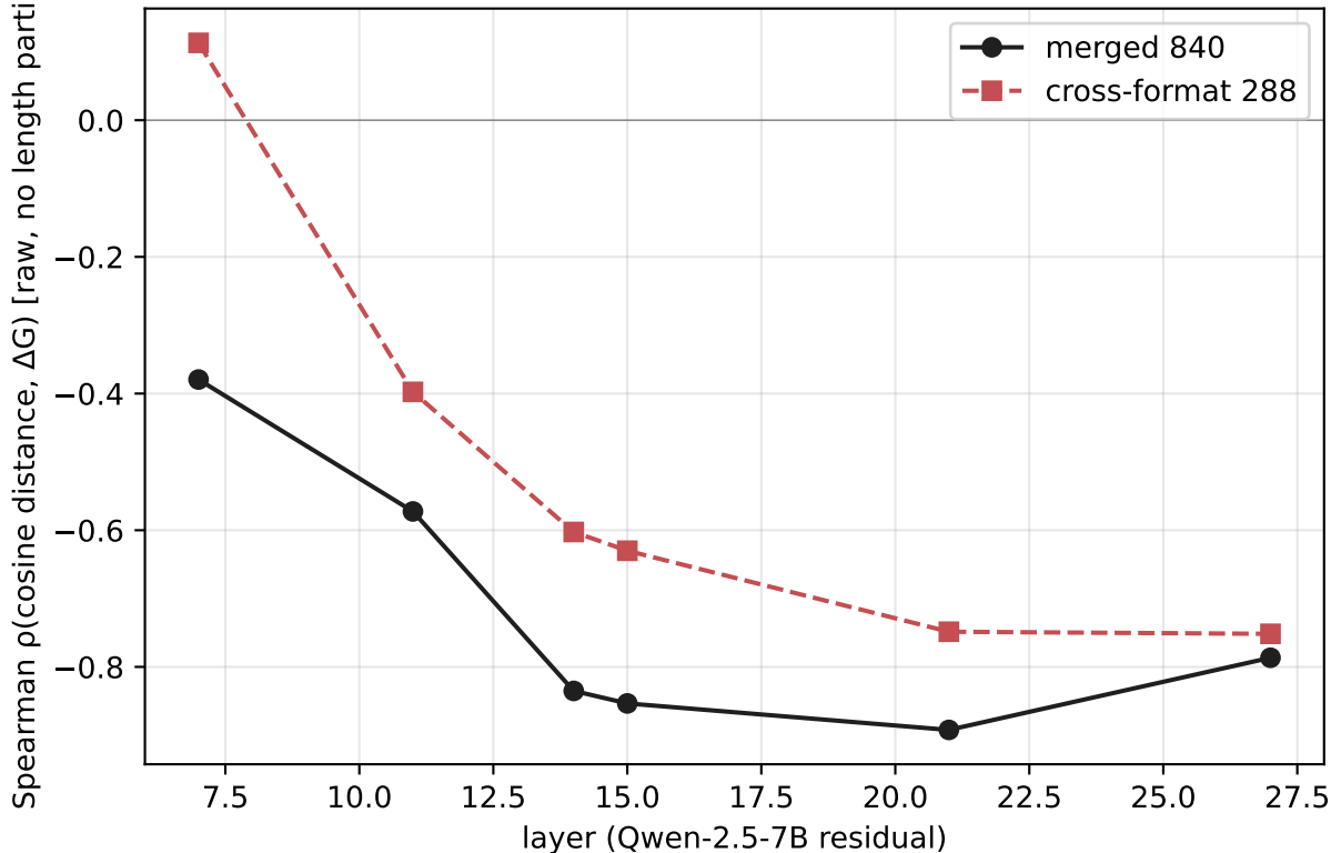
layer-sweep predictor strength
