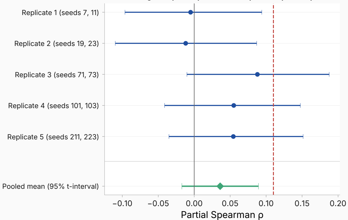
Nearest-negative partial \rho at the no-implant step-5 snapshot
