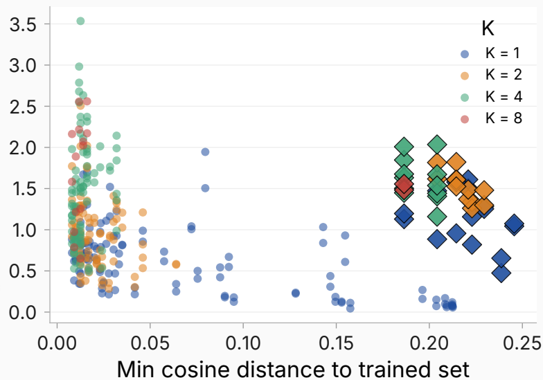
KL vs distance (parallels the hero)
