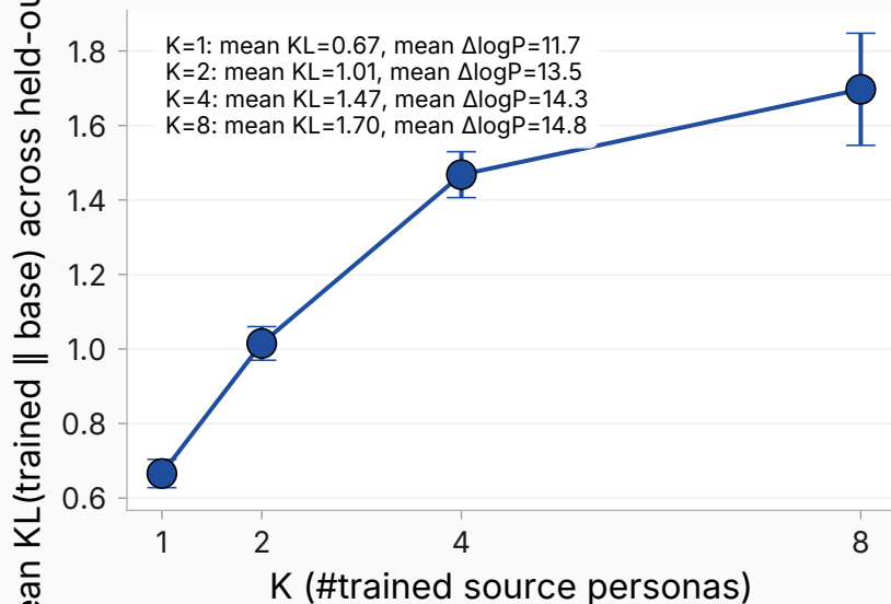
Mean KL rises monotonically with K
